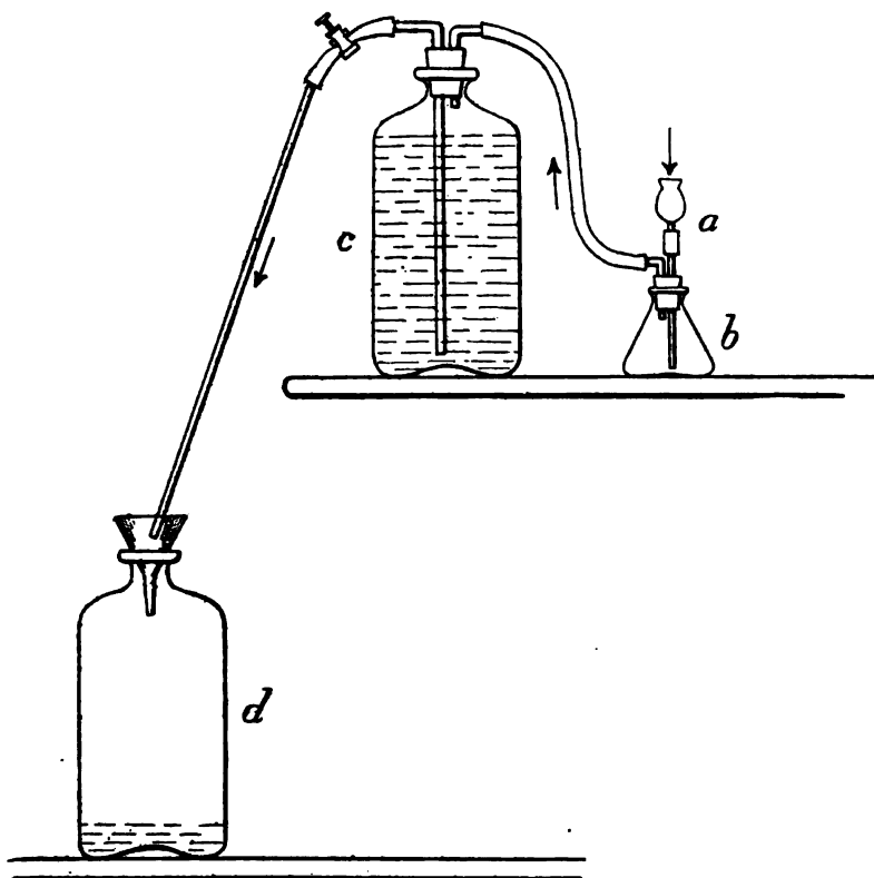
Fig. 2.—Apparatus used in Method II. It consists of : a —a small globe-shaped glass tube containing the glass-wool absorbent for the dust in the air ; b —a small Erlenmeyer flask containing the acidulated permanganate solution to absorb the gaseous organic matter ; c —a graduated flask of eight litres capacity, which serves as an aspirator ; and d —another eight-litre flask into which the water drains from the aspirator.
